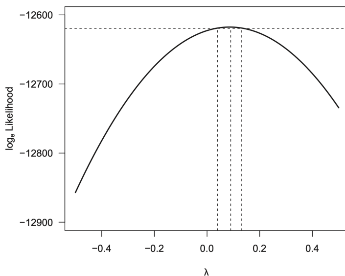
Figure 21.1: Box-Cox transformations for the SLID regression of wages on sex, age, and education. The maximized (profile) log-likelihood is plotted against the transformation parameter \lambda . The intersection of the line near the top of the graph with the profile log-likelihood curve marks off a 95% confidence interval for \lambda . The maximum of the log-likelihood corresponds to the MLE of \lambda . JF Figure 12.14.
