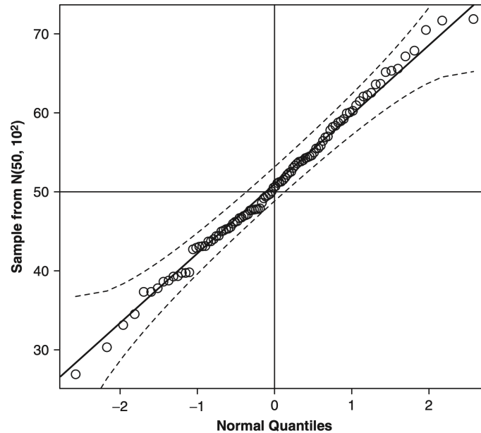
Figure 21.3: Normal quantile-comparison plot for a sample of 100 observations drawn from a normal distribution with mean 50 and standard deviation 10. The fitted line is through the quartiles of the distribution, the broken lines give a pointwise 95% confidence interval around the fit. JF Figure 3.8.
