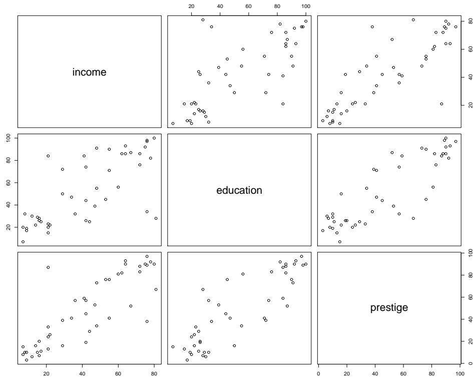
Figure 12.1: Scatterplot matrix for occupational prestige, level of education, and level of income of 45 U.S. occupations in 1950.
